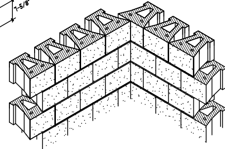
ISOMETRIC WALL SECTION INSIDE CORNER
