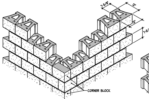
ISOMETRIC WALL SECTION OUTSIDE CORNER
