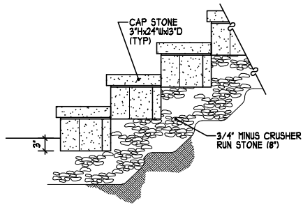
SECTION DETAIL
