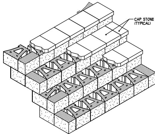
ISOMETRIC STAIR SECTION
